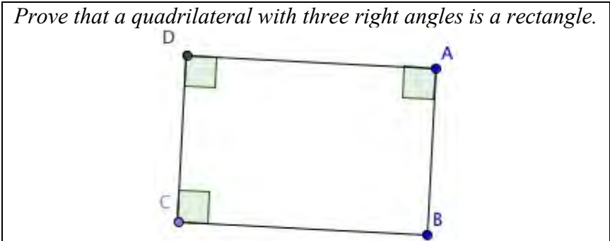
Figure 2: the rectangle problem
